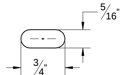
SLOT GEOMETRY
